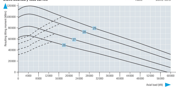
Static boundary load curves
