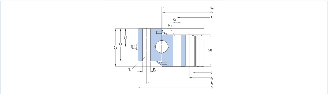
skf-p074-outline-drawing.webp
