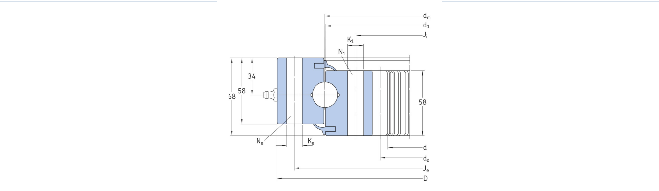
skf-p074-outline-drawing.webp
