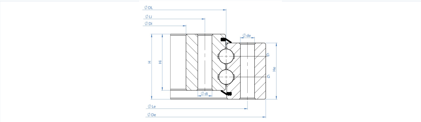
double_row_ball_ungeared-drawing.webp
