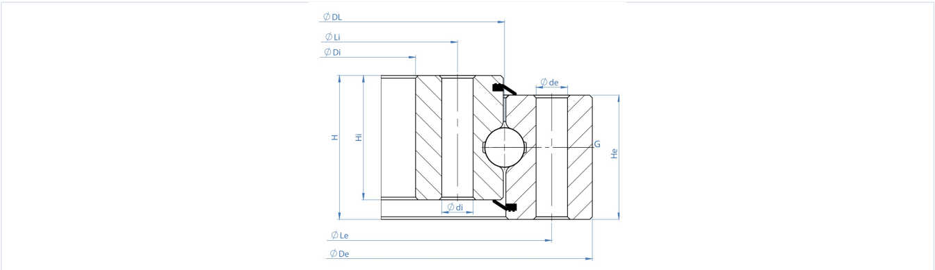
four_point_ungeared-drawing.webp
