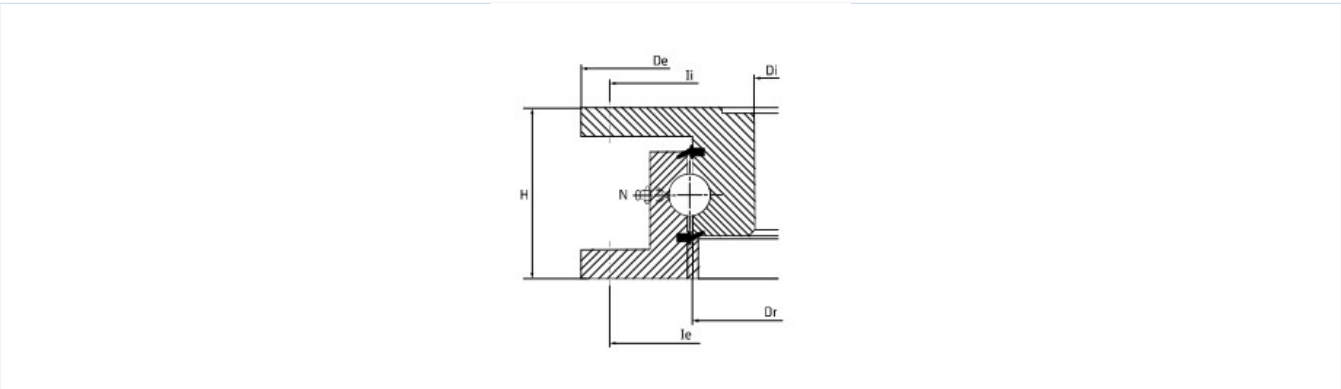
la-leonessa-u-ungeared-drawing.webp
