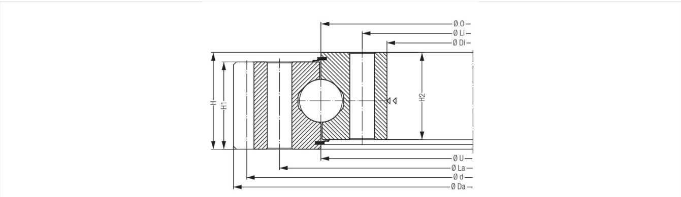
liebherr-page-083-drawing.webp
