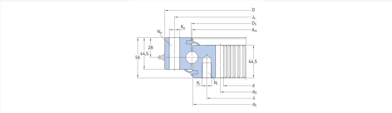
skf-p072-outline-drawing.webp
