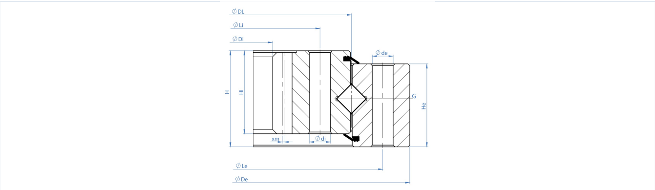
single_row_roller_internal-drawing.webp
