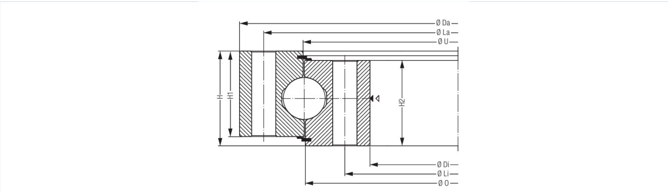
liebherr-page-093-drawing.webp
