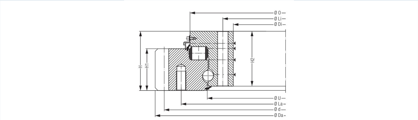
liebherr-page-152-drawing.webp
