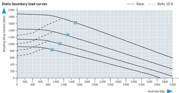
Static boundary load curves
